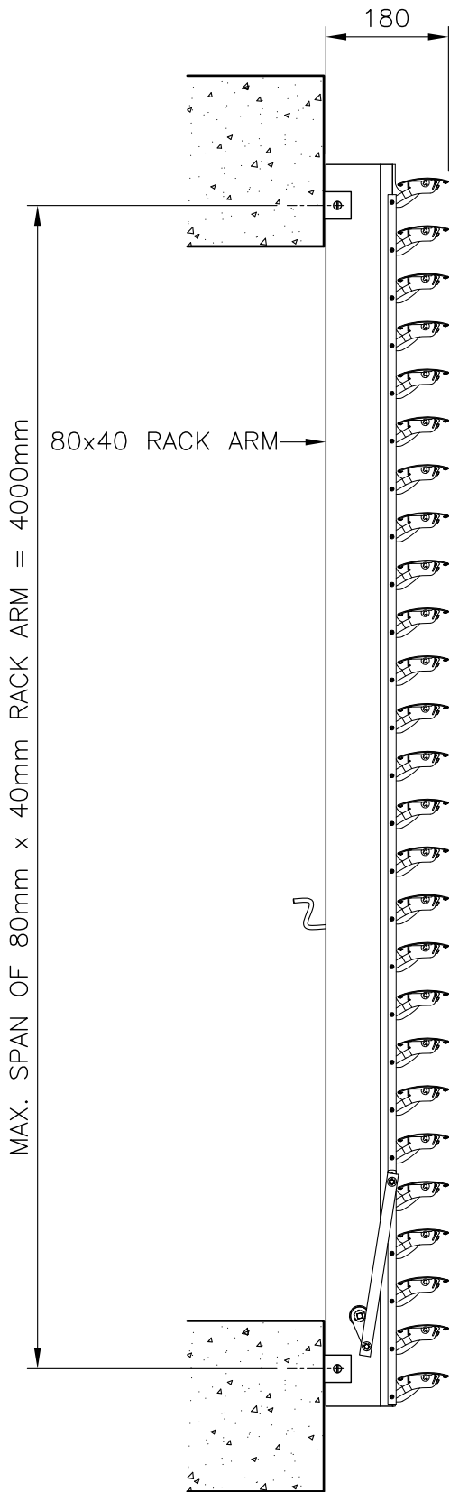
CONTINUOUS LOUVRE WITH 80mm x 40mm RACK ARMS
