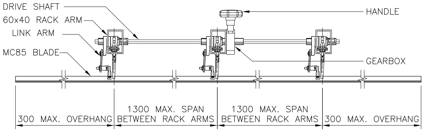
PLAN VIEW (BLADES CLOSED)
