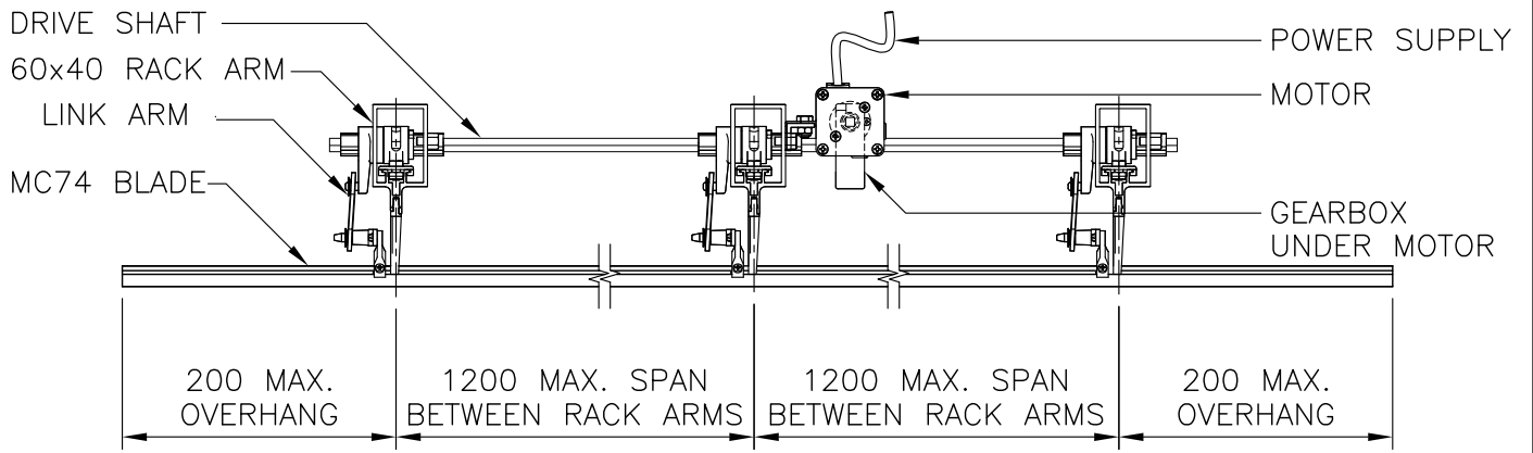
PLAN VIEW (BLADES CLOSED)
