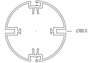
TUBE 80mm
