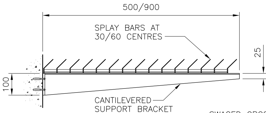
SECTION VIEW
