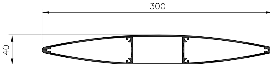
MF300 FIN BLADE EXTRUDED ALUMINIUM
