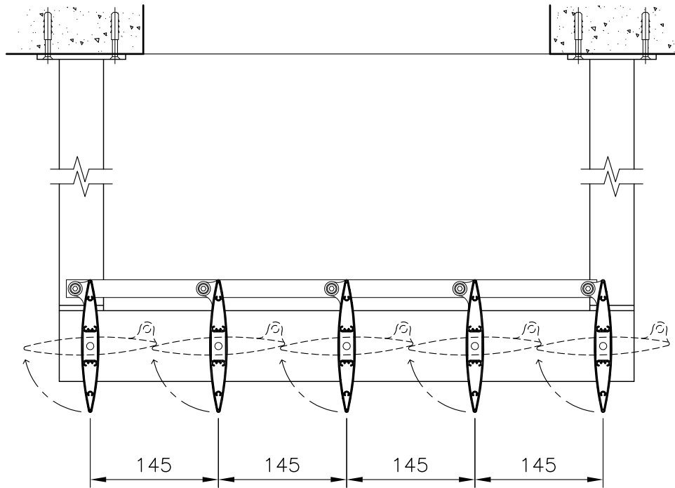
PLAN SECTION
