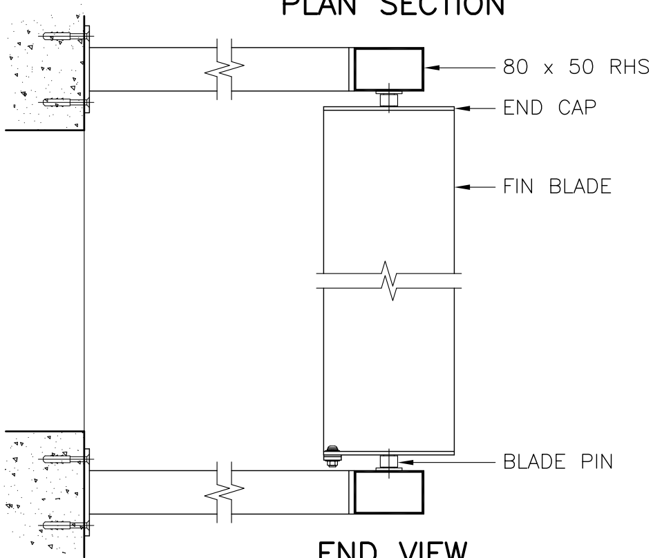
PLAN SECTION
