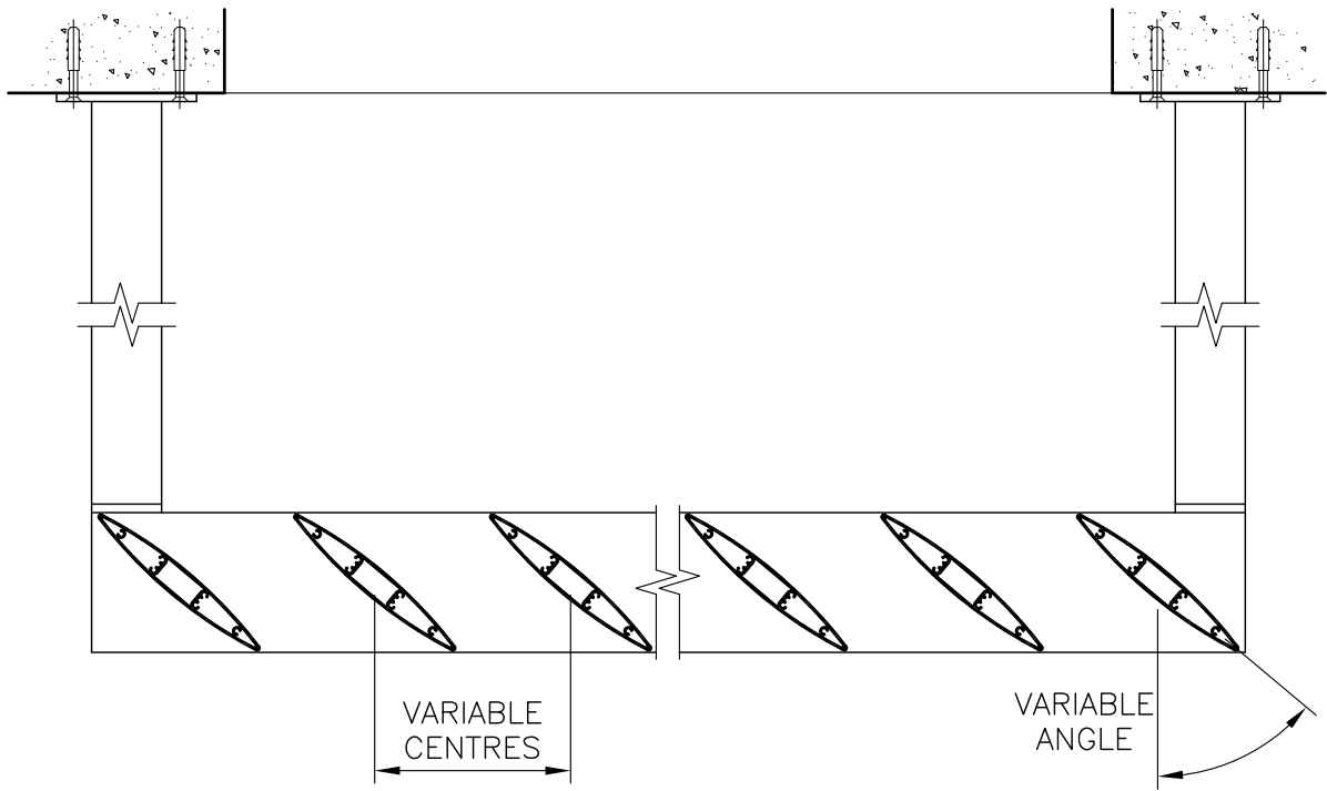
PLAN SECTION
