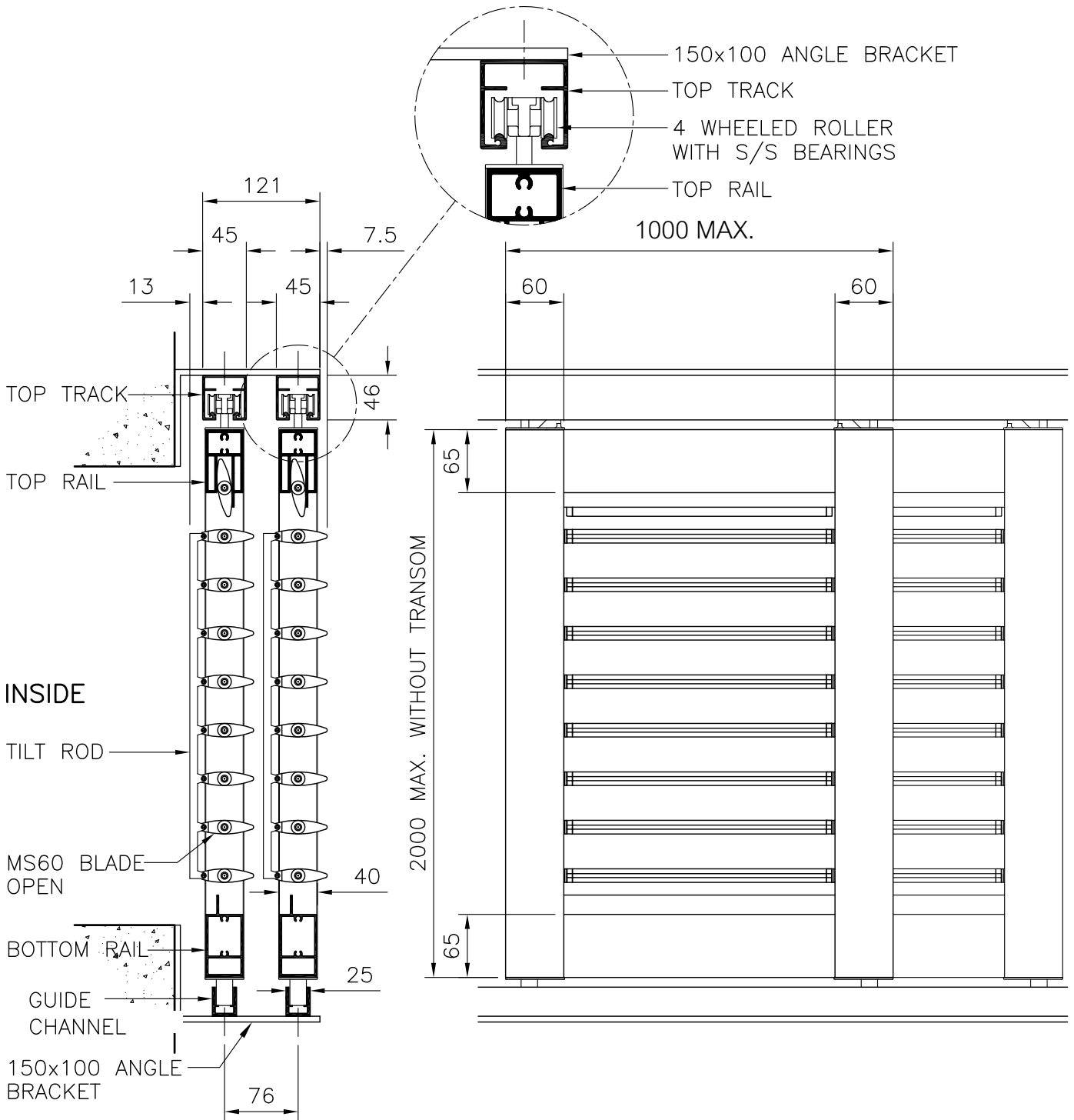
SECTION
